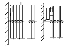
Expandable Panel - Seal to Wall used with even numbered panel openings. Seal to single panel with odd numbered panel openings.
