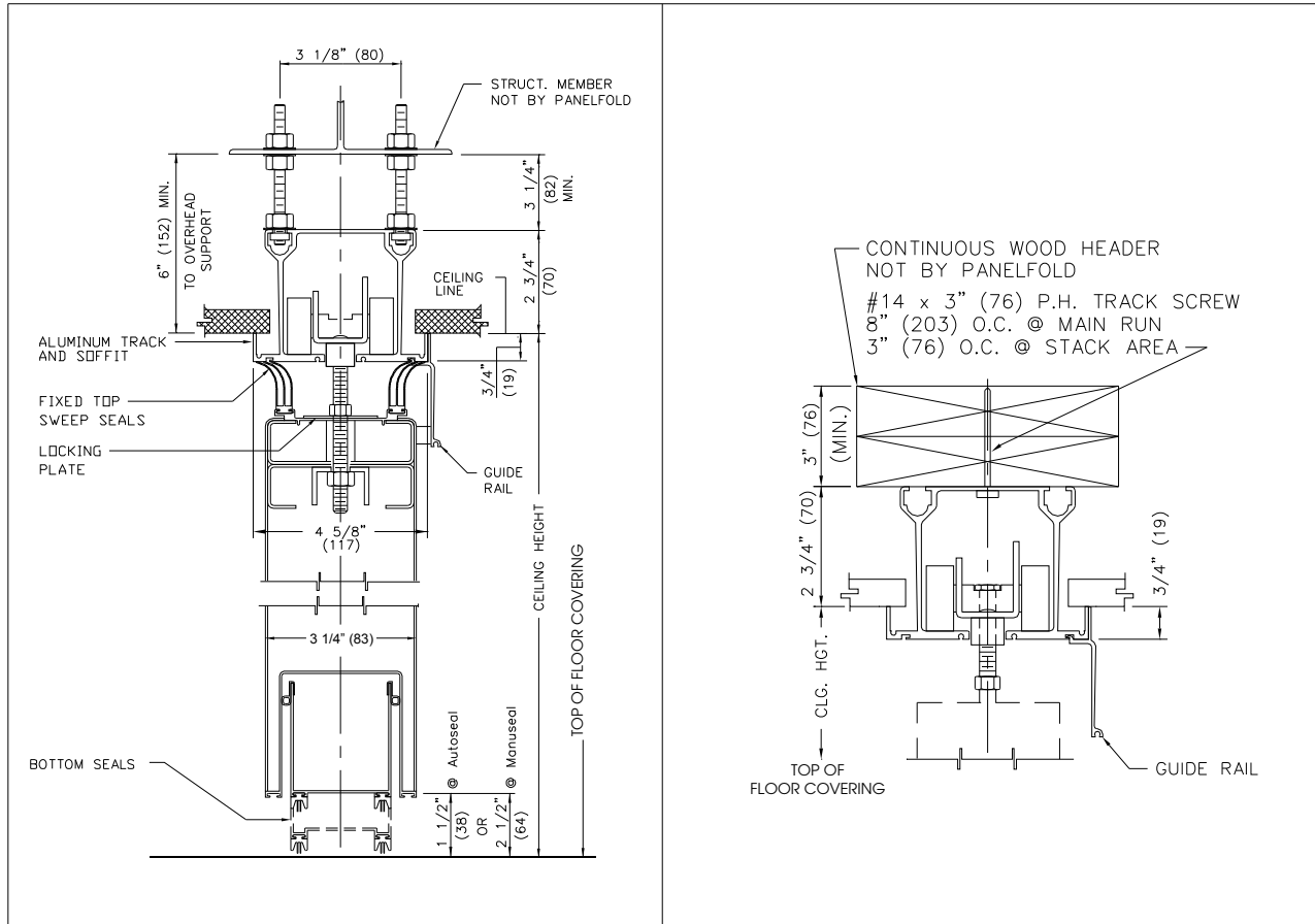
TYPE 7/8 TRACK HANGER ROD SUSPENSION
