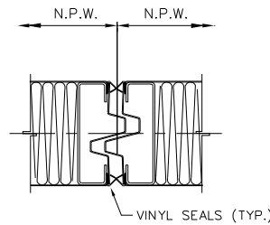
(E) INTERLOCK
