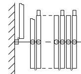
Communicating Panel used with odd numbered panel openings for egress.
